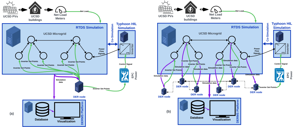
Figure 2: Schematic diagram of the DERConnect testbed components to simulate UCSD microgrid operation for a) centralized voltage regulation and b) distributed voltage regulation. Purple and green arrows indicate data and communication transfer facilitated by DERMS. Execution of the simulation involves three parallel processes. The first includes set point calculation which depends on reading from UCSD PVs and meters then sending those set points to RTDS and EPC Power. The second and third are the two simulators, RTDS and Typhoon HIL, running in parallel.
