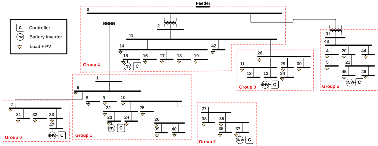
Figure 1: Block diagram of grouping of the UCSD microgrid for the distributed voltage regulation algorithm.
