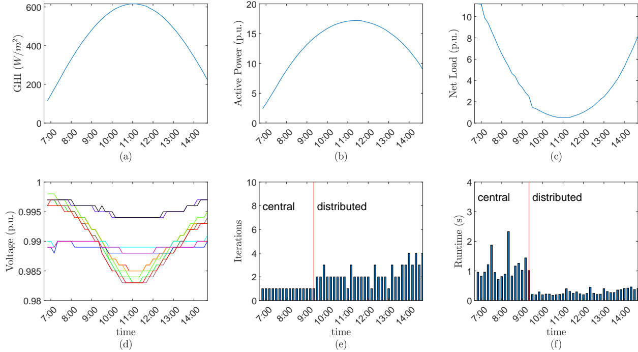
Figure 7: a) Daily profile of solar irradiance for the UCSD area on January 1, 2022 from the National Solar Radiation Database. b) Modeled solar power generation. c) Aggregated net load on the modeled microgrid. d) Voltage profile response for a select group of nodes in the modeled microgrid (bus 6 in red, bus 5 in pink, bus 8 in orange, bus 13 in purple, bus 17 in light blue, bus 24 in green, bus 33 in light green, bus 36 in black, bus 39 in brown, and bus 46 in blue). e) Number of iterations and f) runtime required for convergence of the voltage regulation algorithm. Regulation signals for the first 15 time steps until 0900 h are calculated by the centralized algorithm, afterward setpoints are calculated by the distributed version.
