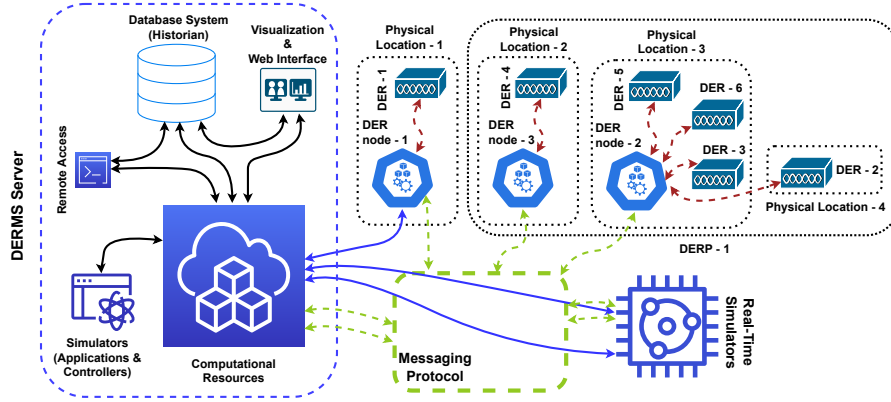
Figure 3: DERMS architecture: Layout of the main components and communication protocols.
