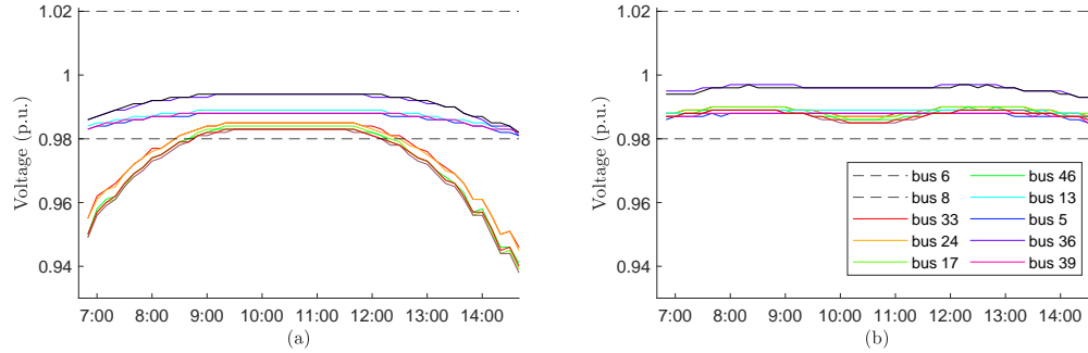
Figure 5: Artificial test case to check the effectiveness of the voltage regulation at select buses. a) without the voltage regulation and b) with the application of the voltage regulation.
