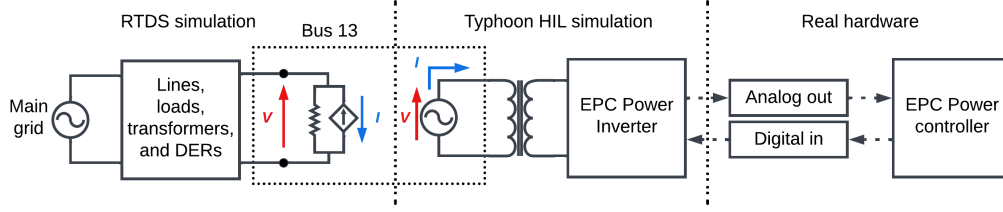
Figure 4: Simplified circuit diagram for the integrated real-time simulation. The UCSD microgrid model is decoupled at bus 13 and the two sub-circuits are separately simulated in the RTDS and Typhoon HIL. Voltage and current at bus 13 are synchronized between both simulators for consistent operation.
